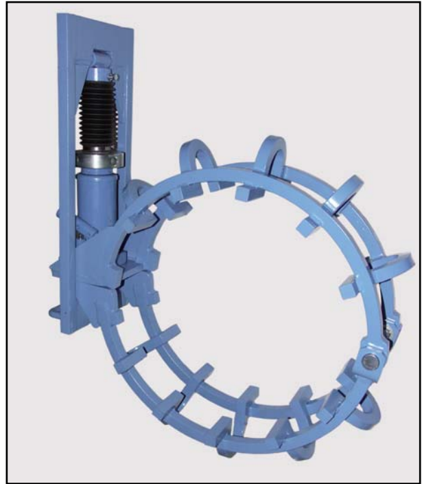
External line-up clamps heavy-duty DN 700/28"
