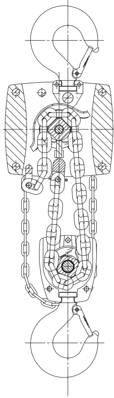
Yalelift 5t
