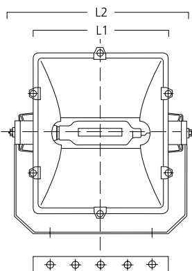
FMD 2000 5 holes Ø16.5mm
