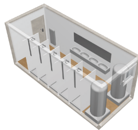
DUSCH-CONTAINER
